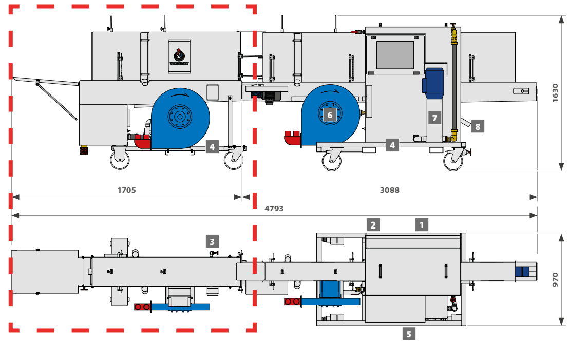
TUNNEL FOR DISINFECTON (accessory)
