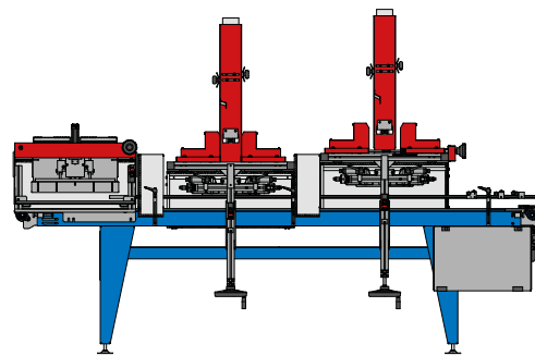
ND 3300 with 3 mov. denester for barquette and double denester for godet.
