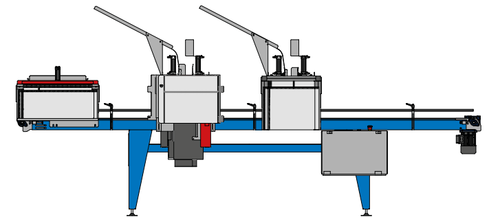
ND 4300 with 3 mov. denester for thermoformed trays, 3 mov. denester for thermoformed packs and ETC2 labelling machine, 3 mov. denester for pots.
