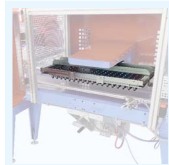
8 Plate dibbler mod. NI for depth bigger than 20 mm and for seeders assembled with nr. 3 sowing drums.
