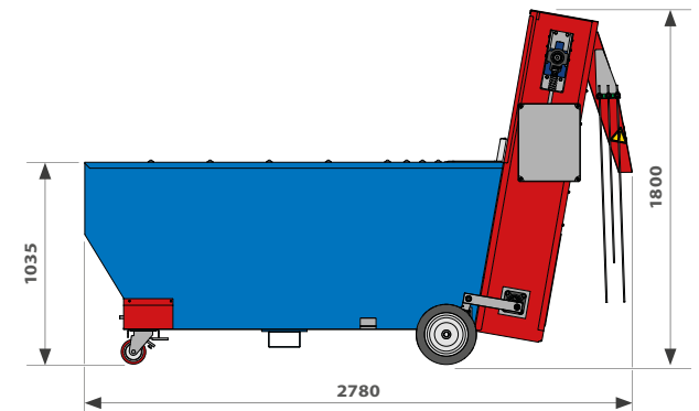
TR1800 as soil hopper, placed between CARBB and RN12, complete with connecting mod. NTV belt , with special legs and side boards.
